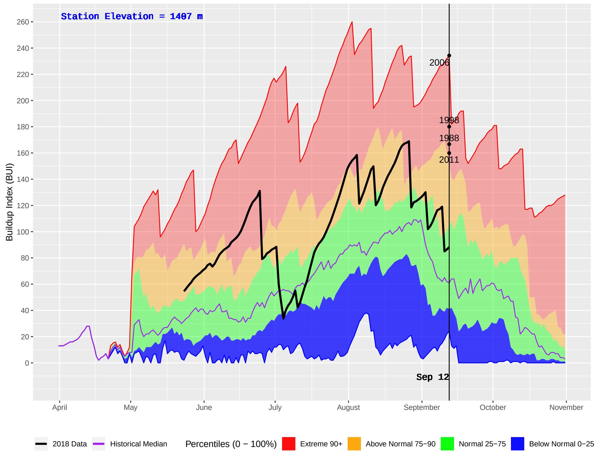
THYNNE (279) : Historical (1977–2016) and Current (2018) Daily Buildup Index (BUI)
