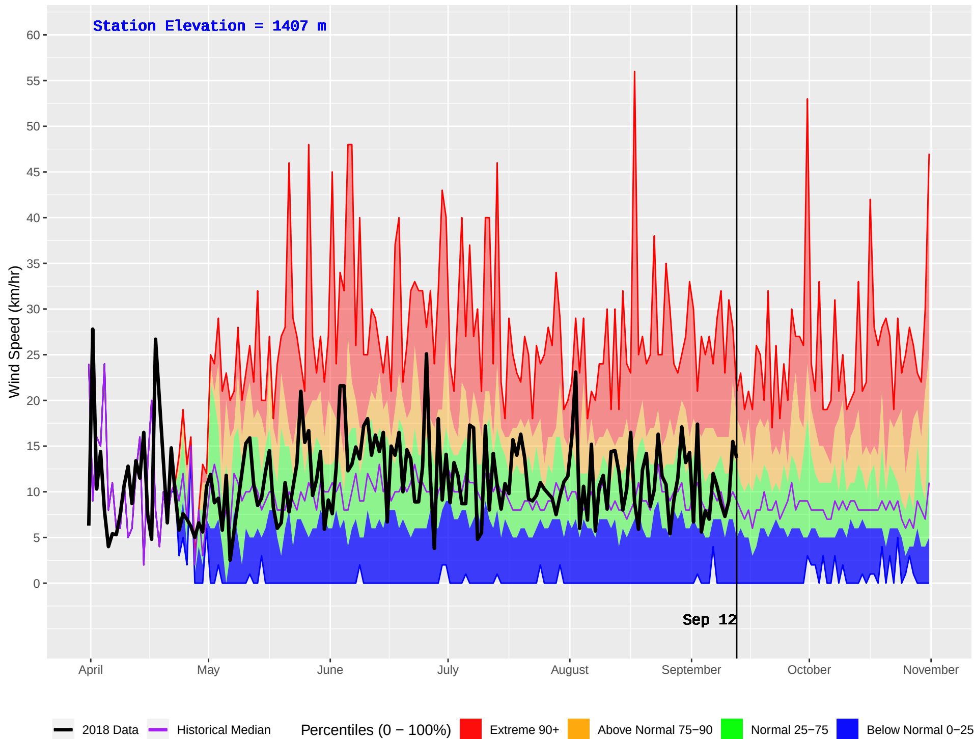
THYNNE (279) : Historical (1977–2016) and Current (2018) Daily Wind Speed
